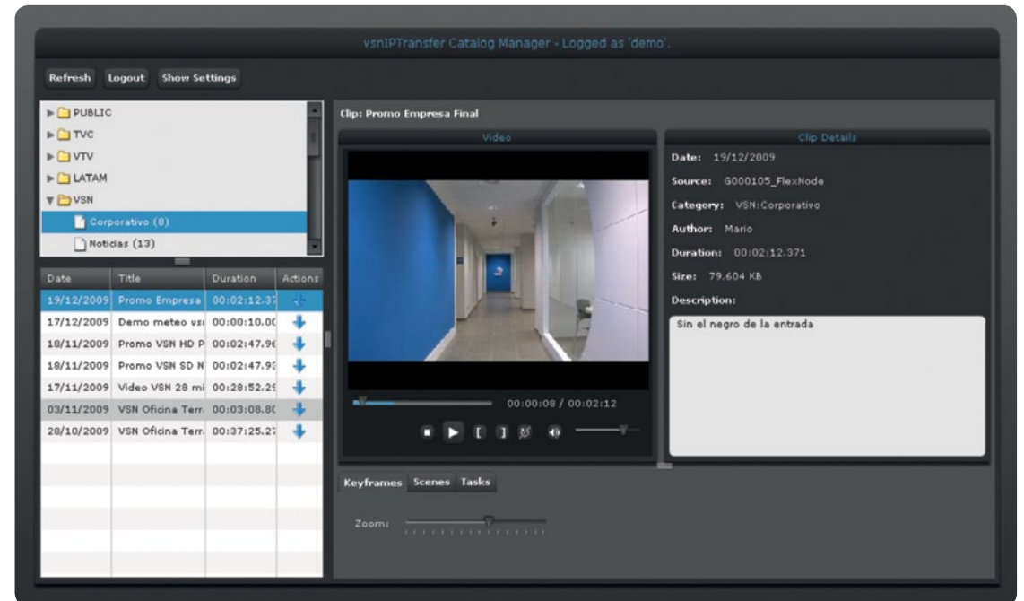
VSNIPTRANSFER screenshot
